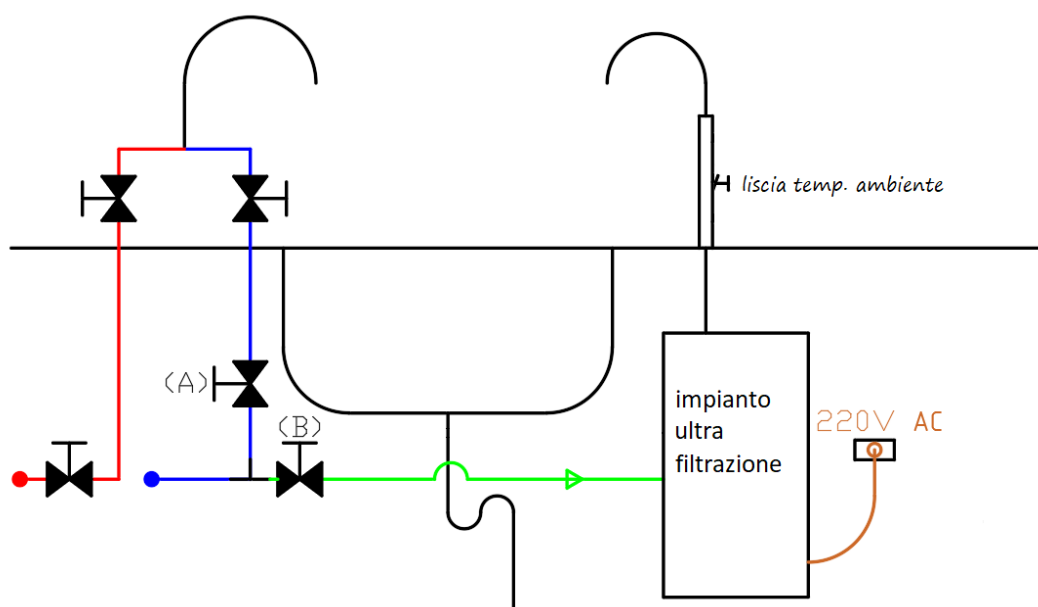
Figura 5a – C100UF
